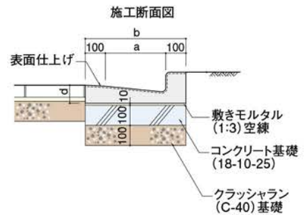
[L型側溝]
